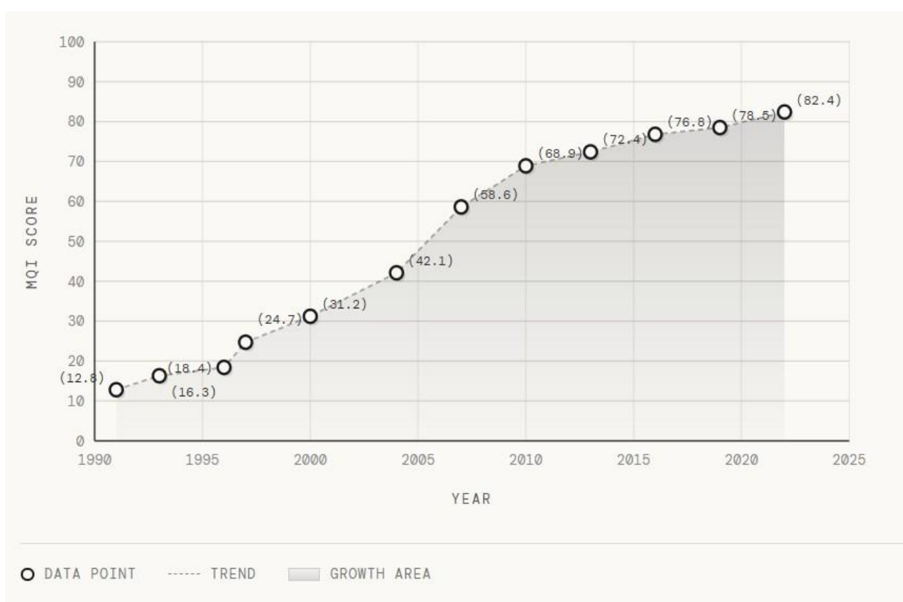
Figure 1: Temporal Distribution of MQI Scores (1991-2023)
