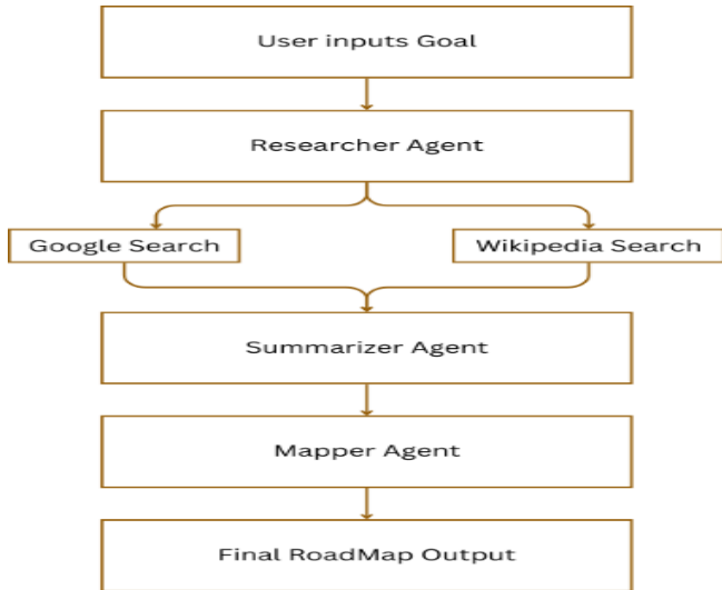
Fig. 3. Process Flow Diagram of PathPro
