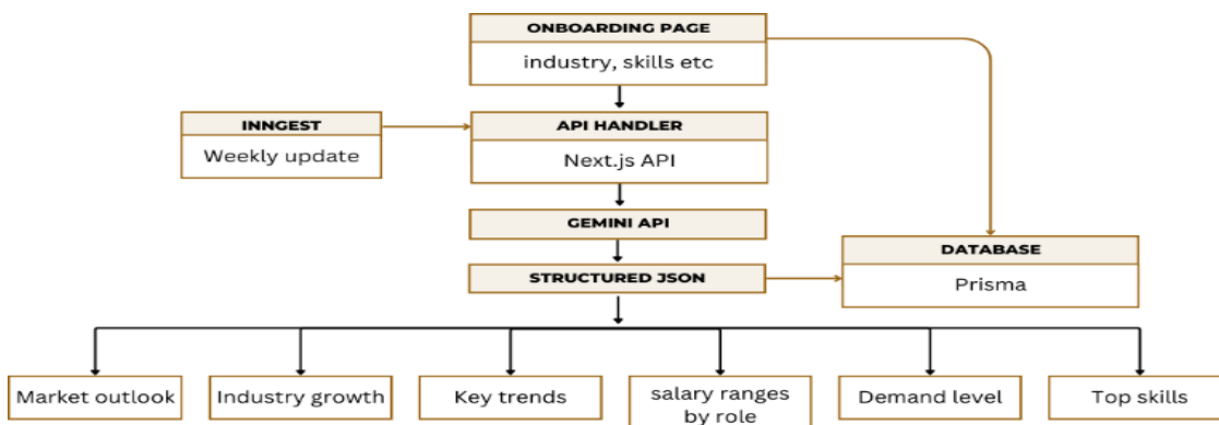
Fig. 4. Process Flow Diagram of TrendLens
