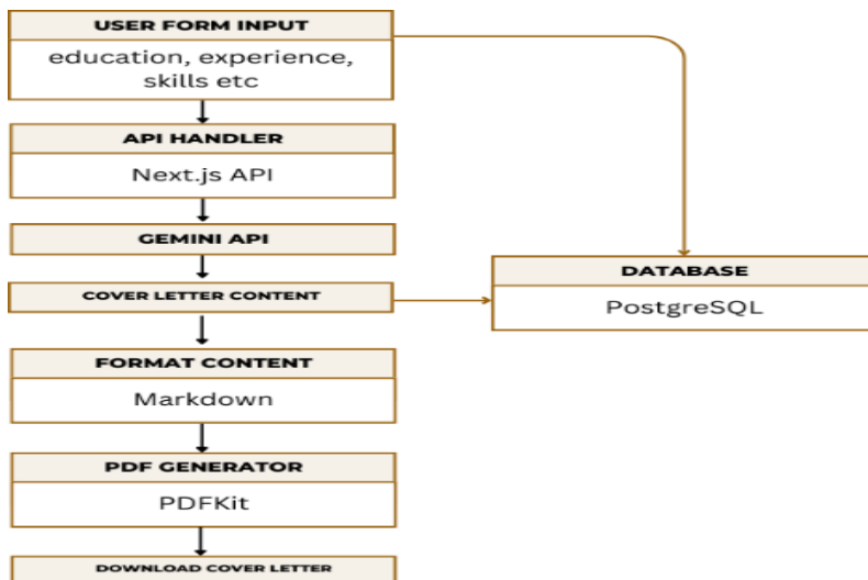
Fig. 6. Process Flow Diagram of CoverForge
