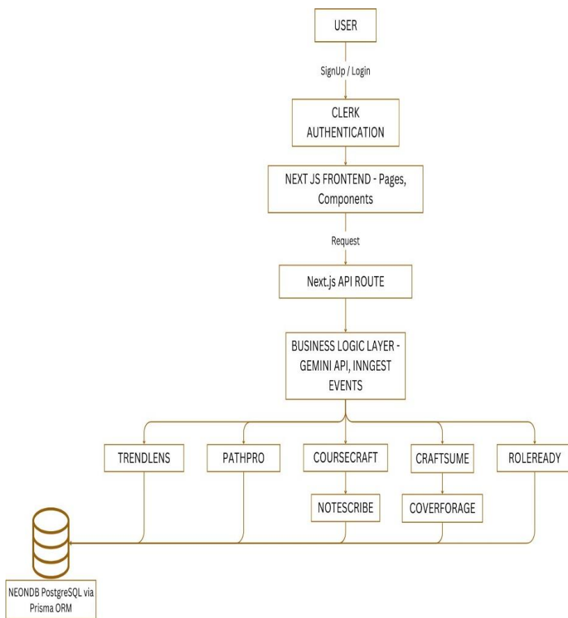
Fig. 1. System Architecture Diagram of AI-Powered Career Accelerator
