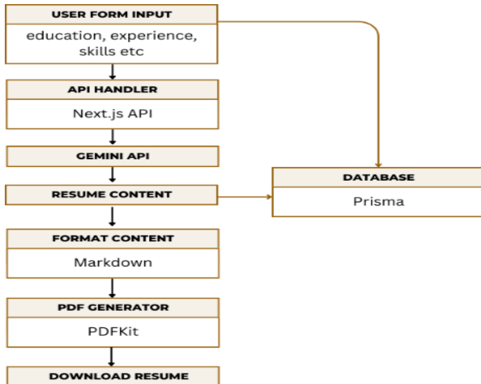
Fig. 5. Process Flow Diagram of Craftsume
