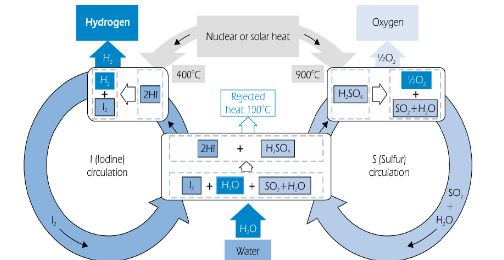
Figure 3. Thermochemical water splitting cycle.
