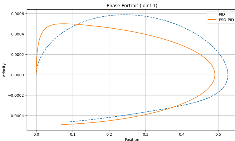
Figure 6: Phase portrait analysis of the joints
