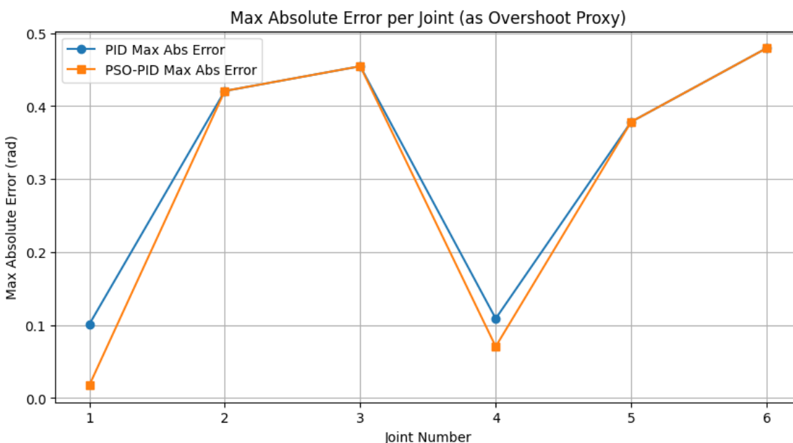
Figure 8: Comparative MAE results
