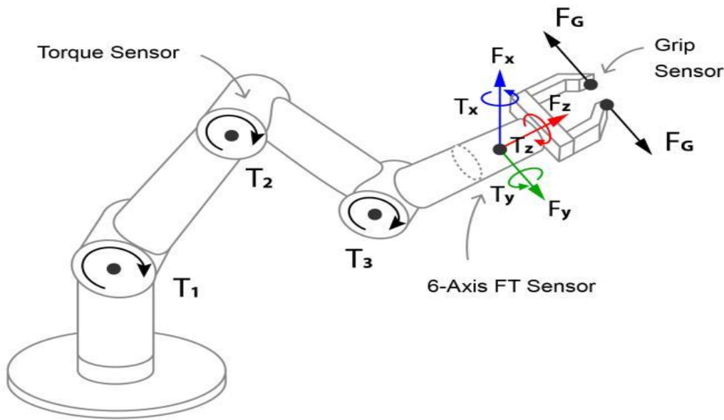
Figure 1: 6-DoF Robot arm with the schematics (Chavez et a., 2023).
