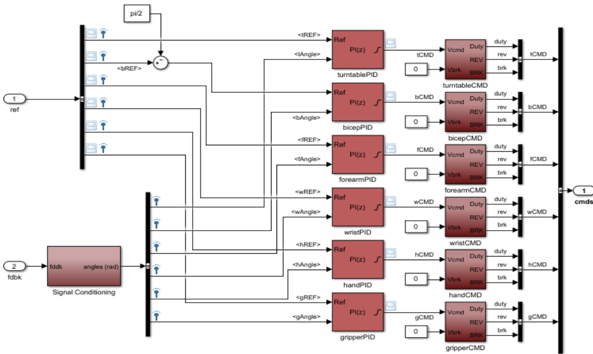
Figure 3: Controller structure in Simulink
