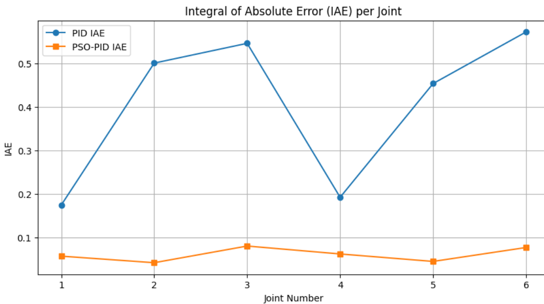
Figure 7: The comparative IAE results
