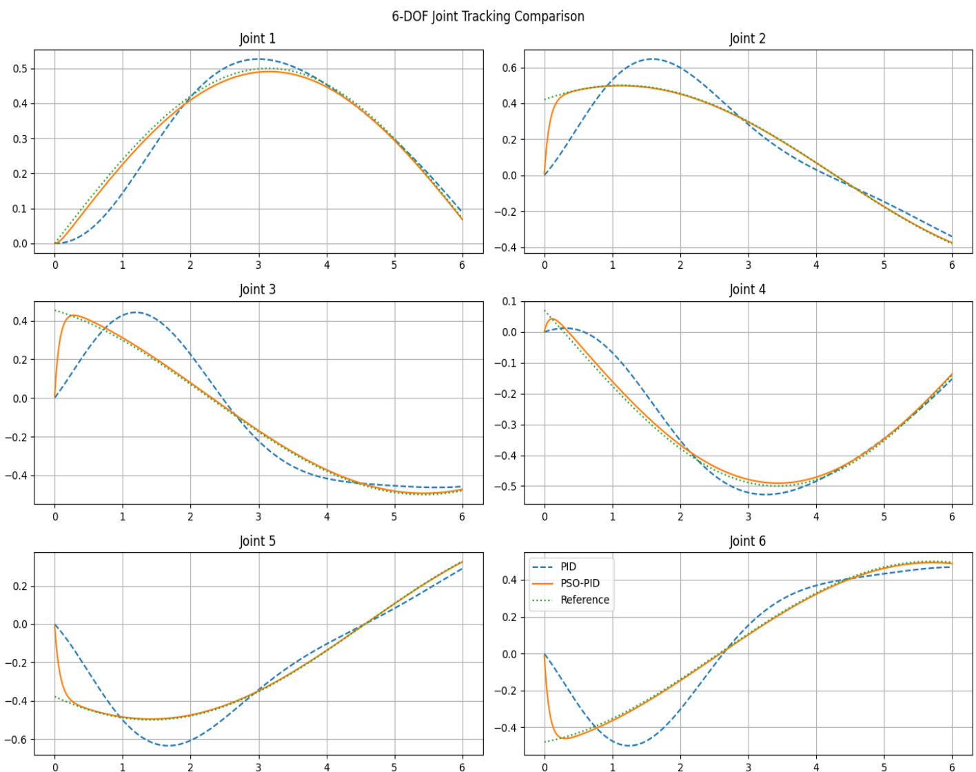
Figure 4: Results of 6DoF tracking comparison
