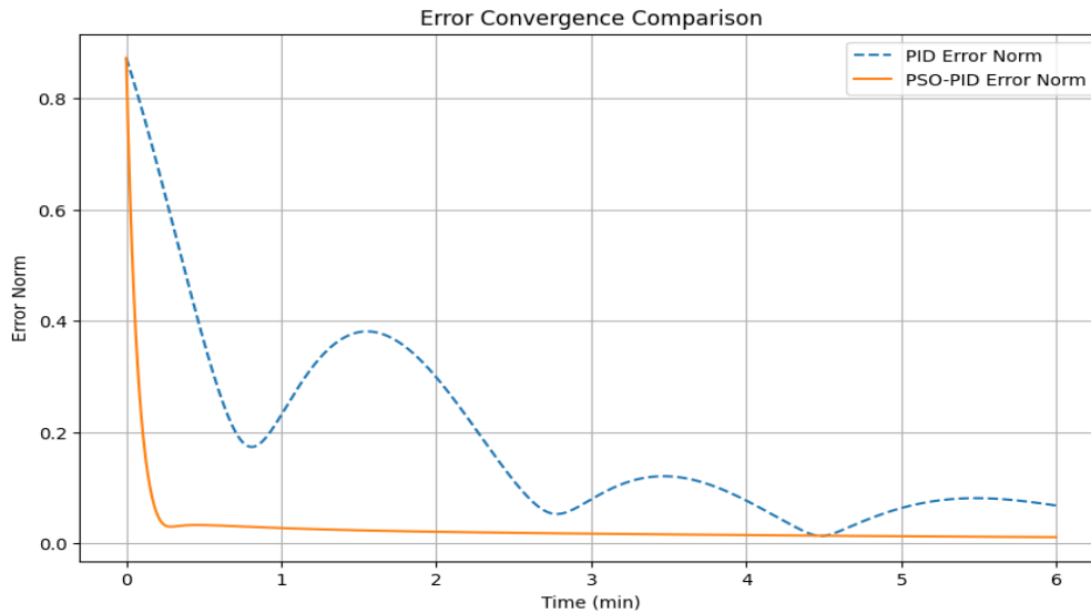
Figure 5: Error convergence comparison
