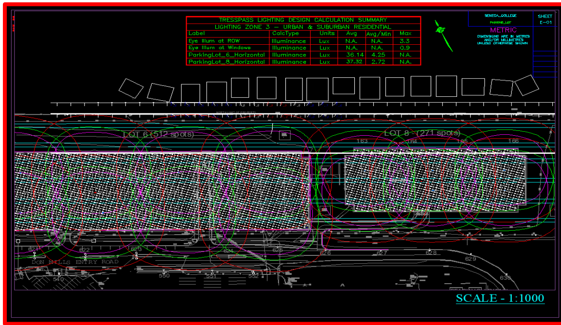
Figure 6. Lighting Calculations at Seneca College.
