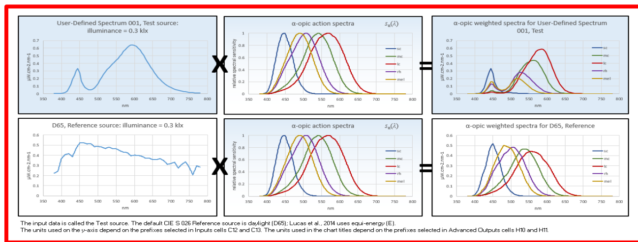
Figure 7. Alpha-Optic Spectral Distribution.
