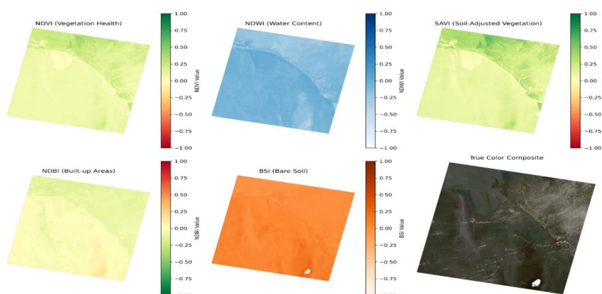
Figure 4: Spatial distribution of spectral indices
