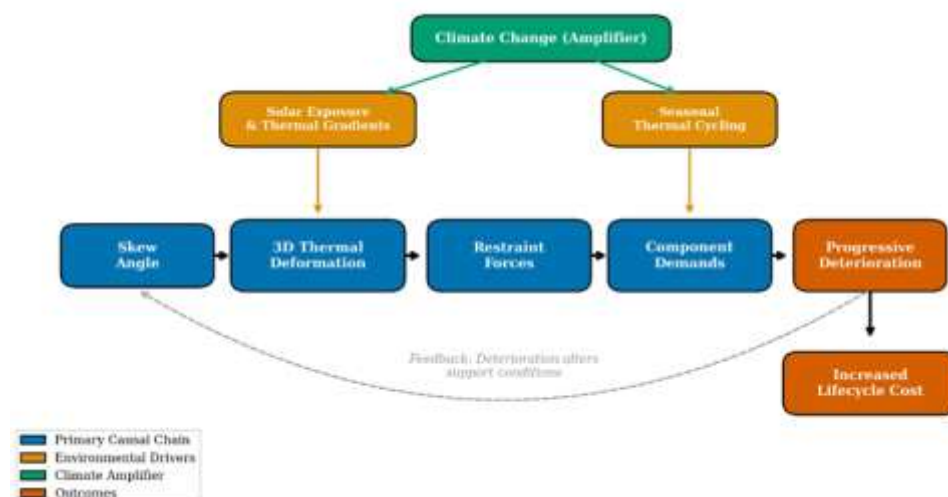
Figure 6: Conceptual framework of environmentally induced behavior in highly skewed bridge superstructures
