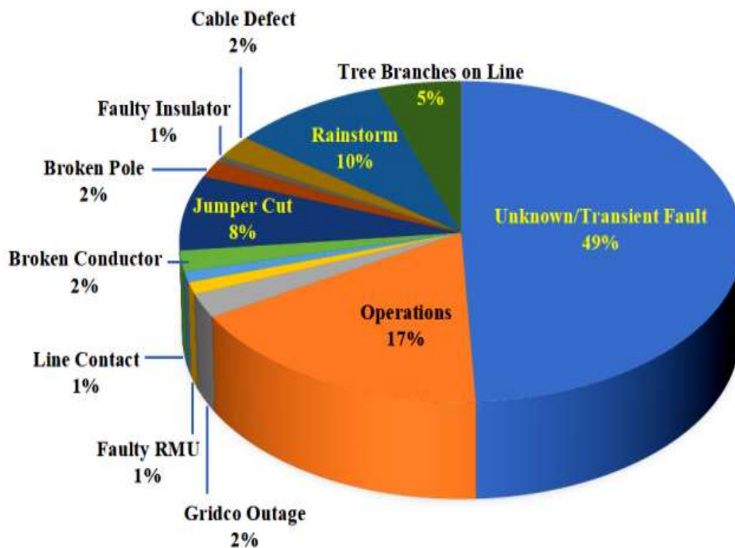
Fig. 12 Faults Causing Customer Interruptions
