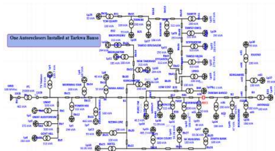
Fig. 14 ETAP Model with One ACR Installed at Tarkwa Banso
